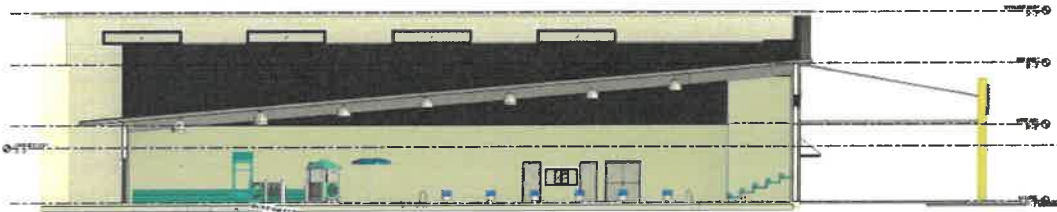
EAST SECTION THROUGH MECHANICAL STORAGE
